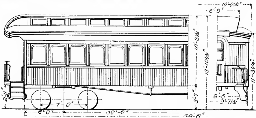
Fig. 157. PASSENGER COACH. BALTIMORE & OHIO RAILROAD. Length, 43 ft. 6 ins. Capacity, 56 persons. Weight, 53,300 lbs. (Details are shown in Figs. 153-160.)
